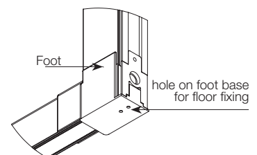
Adjustable floor supports
